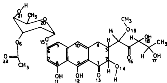
Fig. 2. The reduced model of olivomycin: ASD.
